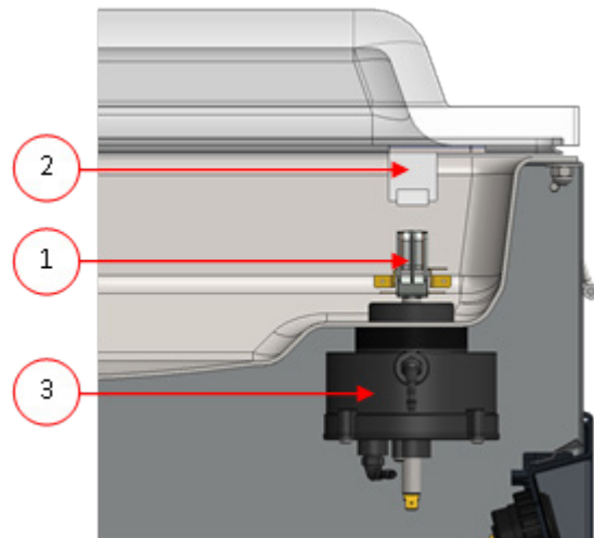
Figure 7: Overview of the Sealing System (Including Sealing Cylinder)
