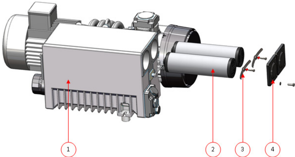
Figure 32: Replacing the Oil Exhaust Filter
