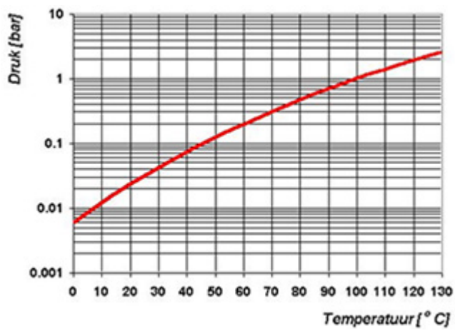
Figure 34: Vapour Pressure Curve of Water
