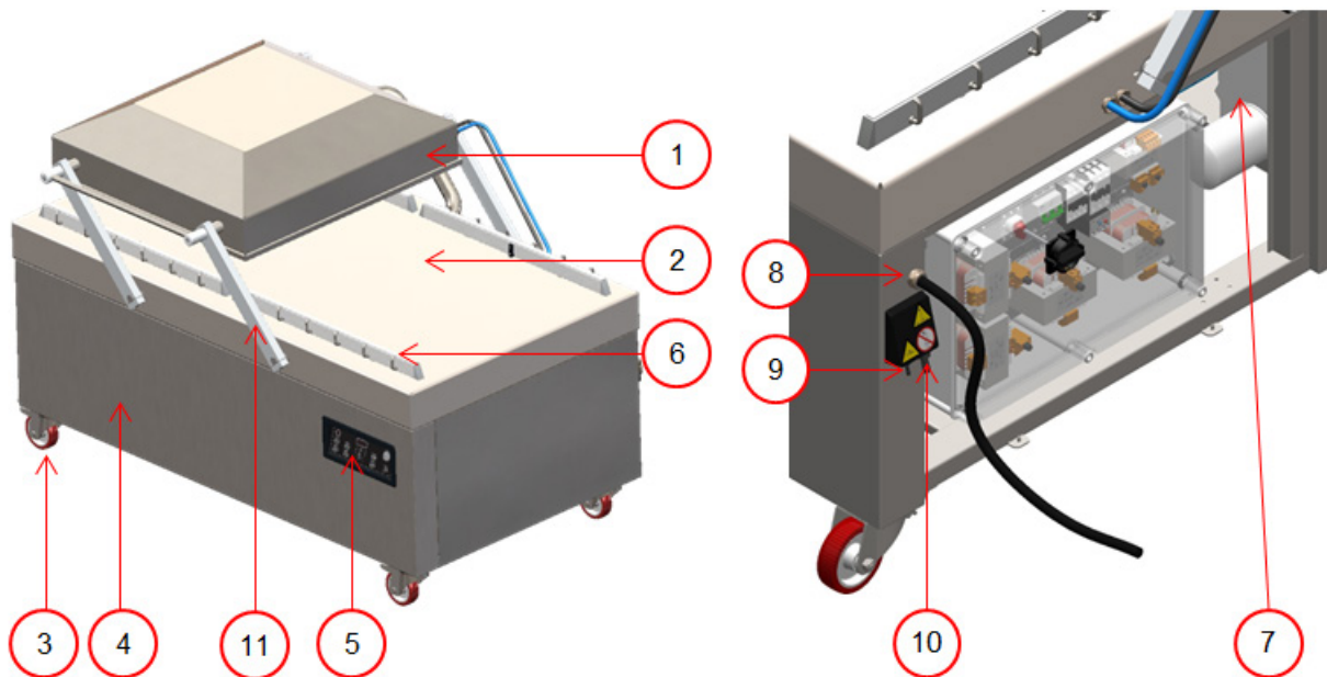
Figure 5: Overview of the Main Components
